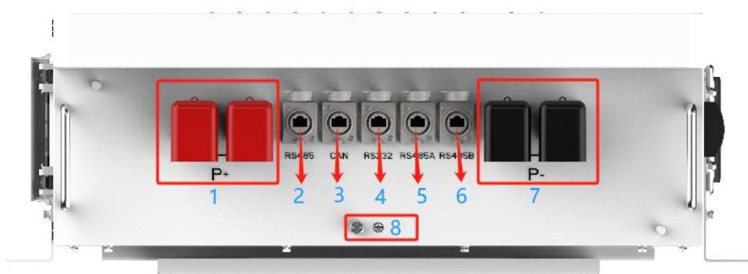
Figure 2 Table1.Battery Pack Front Panel Port Definition
